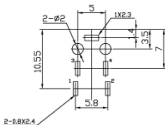
Bottom View \odot
