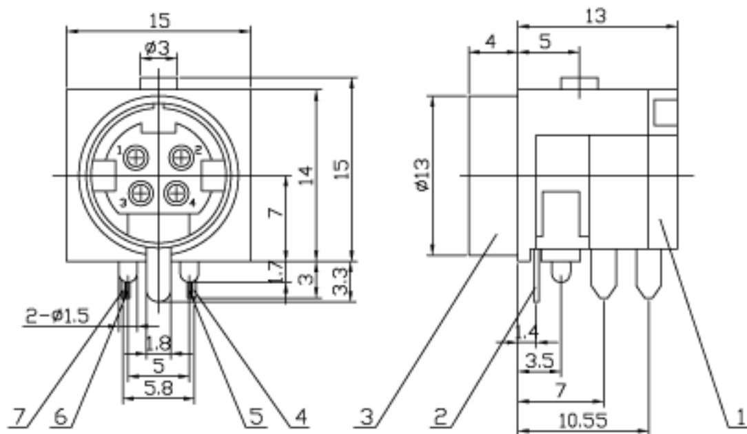
Dimensions of PC board holes (comment)
